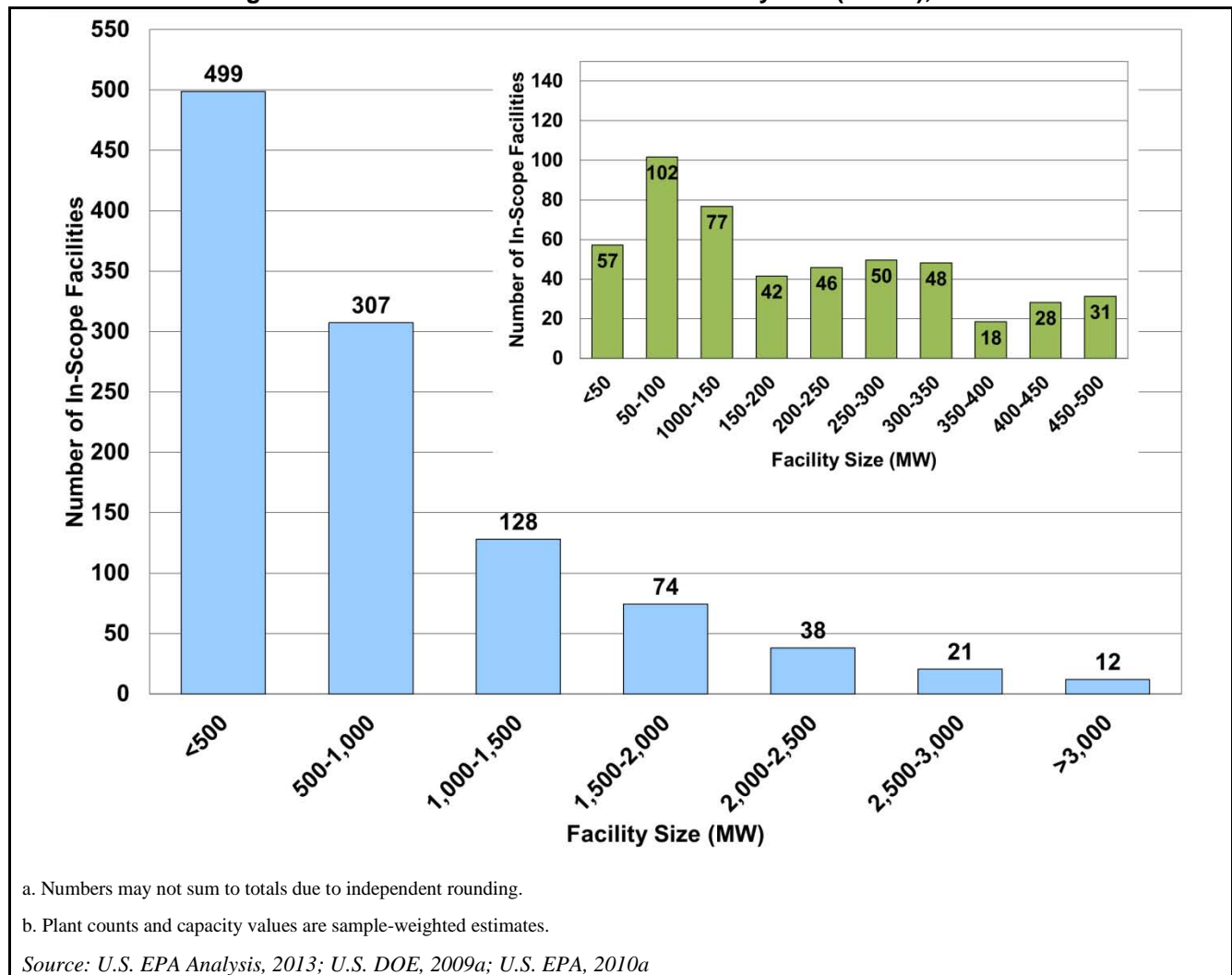
Figure 2-5: Number of Steam Electric Plants by Size (in MW), 2009 a,b
