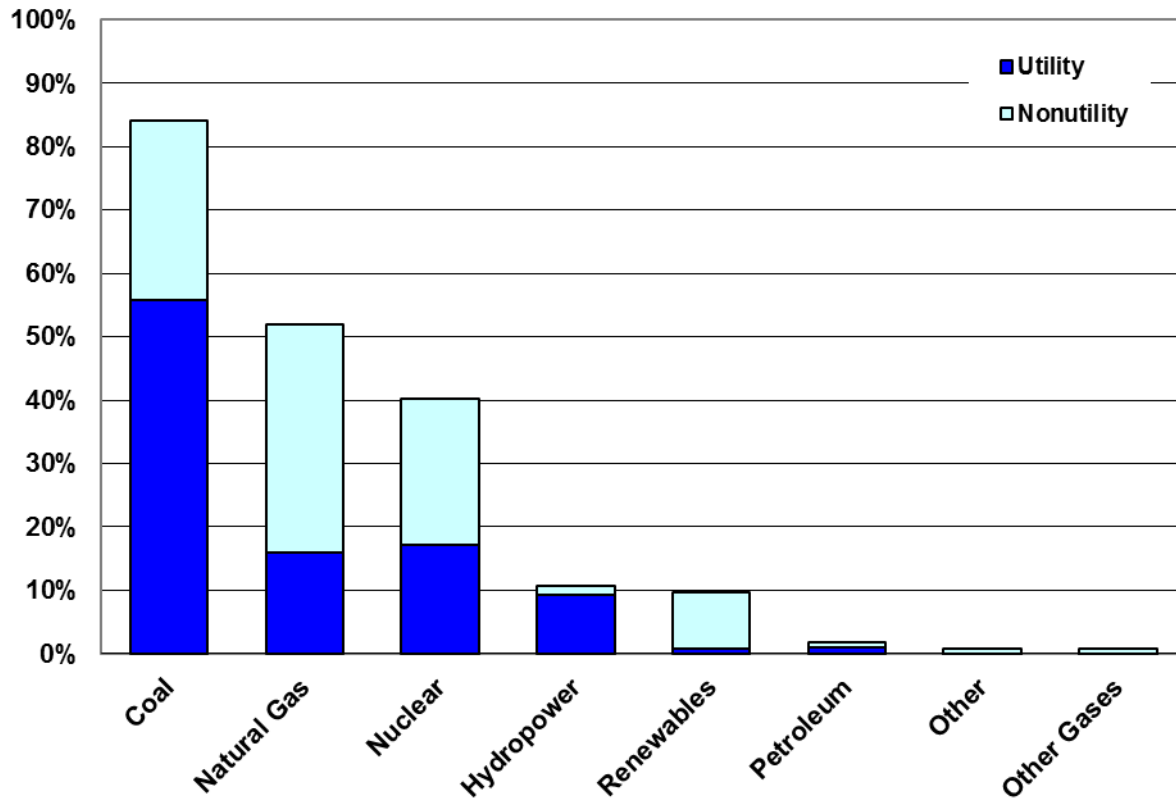
Figure 2-3: Percent of Electricity Generation by Primary Fuel Source and Plant Ownership Type, 2010
